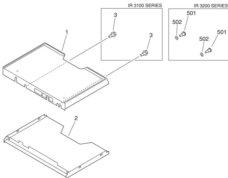
FIGURE G10 DOCUMENT TRAY ASSEMBLY
